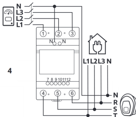
Gavazzi EM340DINAV23XS1PFB
