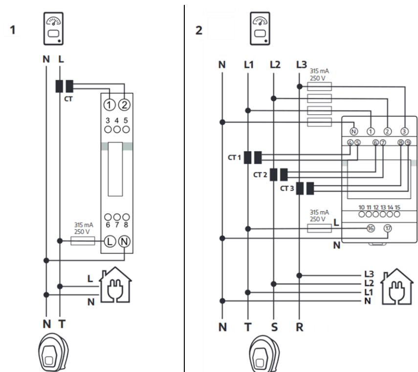
Gavazzi EM111DINAV51XS1X
